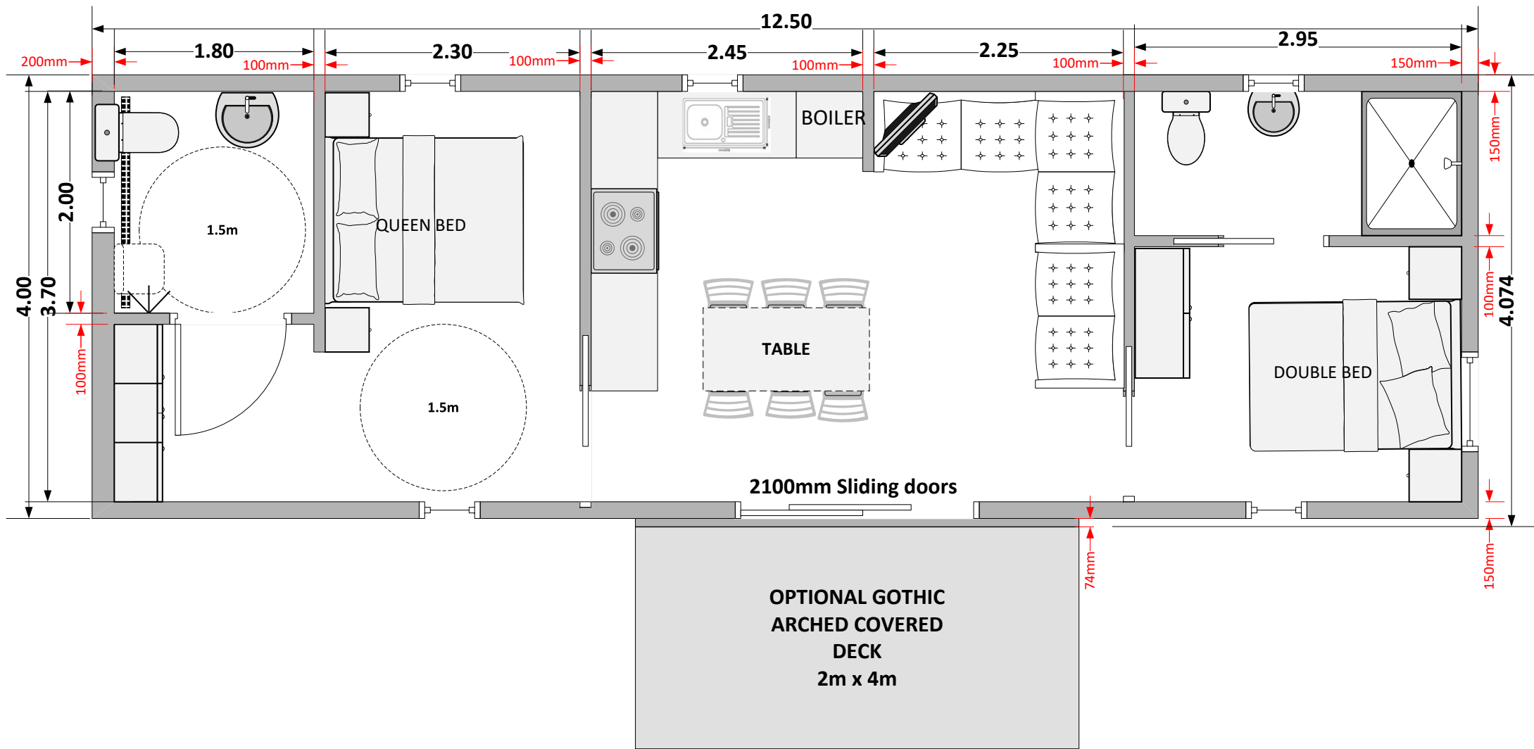
THE OMNIPOD LARGO SIDE ENTRY Internal floor area c.44m 2
